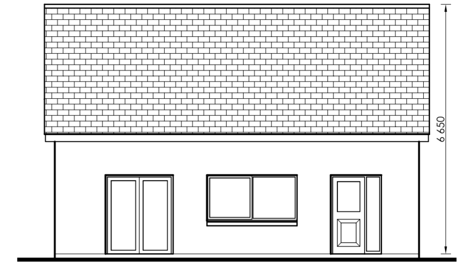
Rear Elevation
